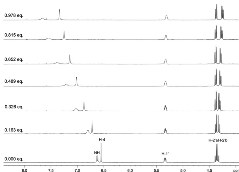
Figure 3. Plots of ^1\text{H} NMR (500 MHz) spectra of 1 on addition of TBACN using \text{CD}_3\text{CN} as solvent.
