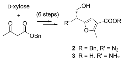
Scheme 1. Stereoselective synthesis of furyl-based amino acids.
