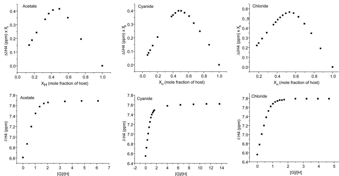
Figure 4. Job plots (top) and ^1\text{H} NMR titration plots (bottom) for the complexation of cyclopeptide 1 with tetrabutylammonium acetate, cyanide and chloride salts in \text{CD}_3\text{CN} solution.
