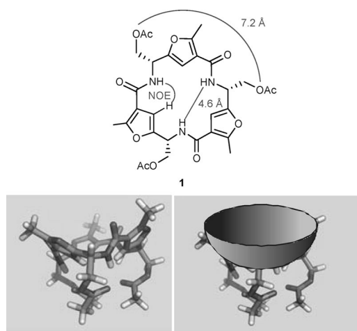
Figure 2. Structural analysis of cyclopeptide 1 by molecular modeling using MacroModel and the MM2* force field.
