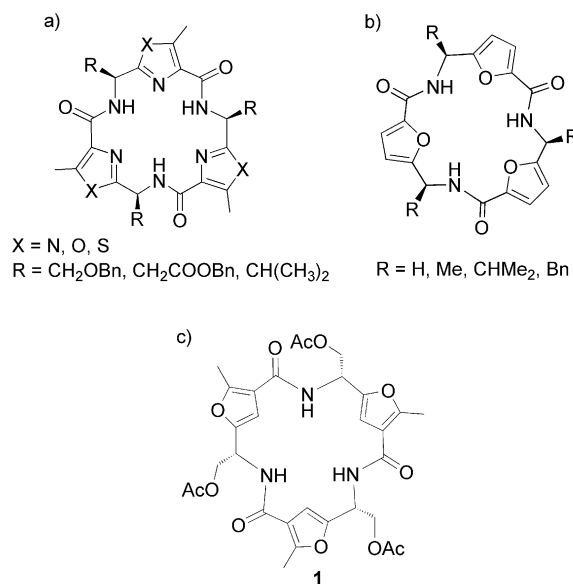
Figure 1. a) Heteroaromatic cyclopeptides as molecular platforms. b) Furyl cyclopeptides as anion binding receptors. c) New furyl cyclopeptide prepared.
