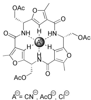
Figure 6. Aryl CH-anion hydrogen bonds in complexation of anions.
