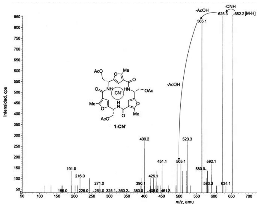
Figure 5. ESI spectra for the complexation of 1 with cyanide.
