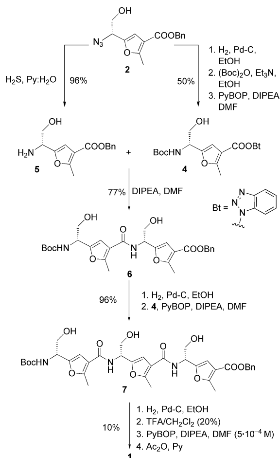
Scheme 2. Synthesis of furyl cyclopeptide 1 .
